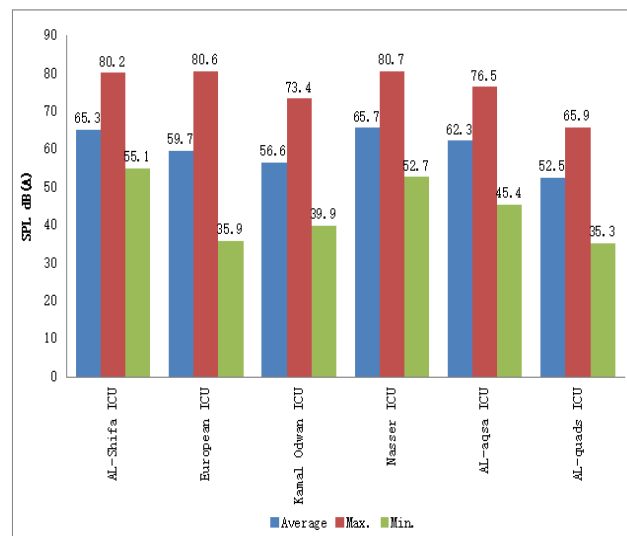
Fig. 1. The average, maximum and minimum values of SPL in all ICUs
