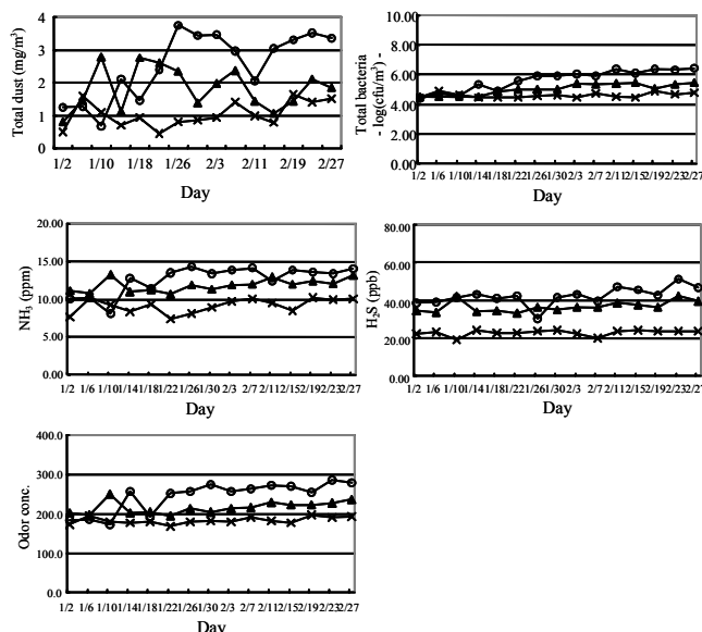
Figure 1. Fluctuation of air pollutants (total dust, total bacteria, \text{NH}_3 , \text{H}_2\text{S} , Odor) in the confined pig house at time (* 8:00-9:00 am, o 2:00-3:00 pm, x 8:00-9:00 pm)
